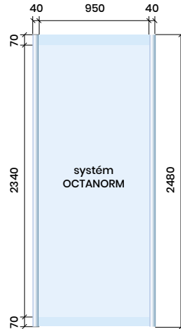
detail panelu
